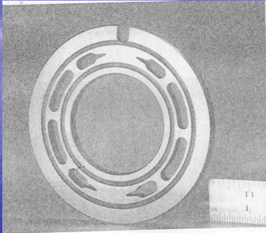
Figure 9.9 Electrochemically machined valve plate (Source: courtesy, Anocut, Inc., Elk Grove Village, Ill.).
