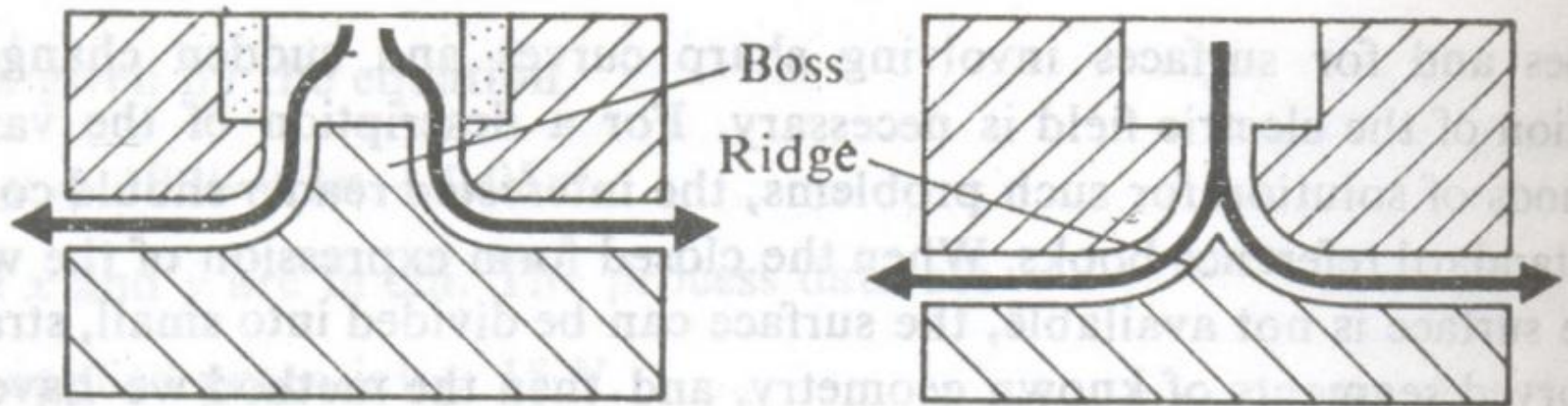
(a) Boss formation
