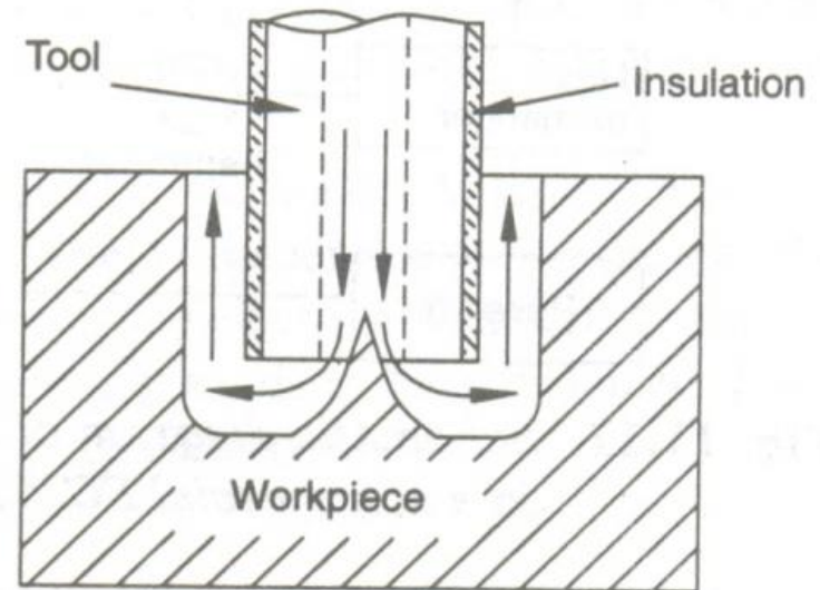
(b) Insulated electrode
