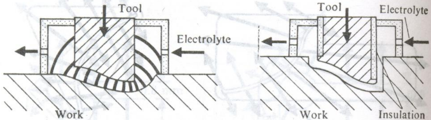
(a) Tool without insulation (b) Insulated tool
