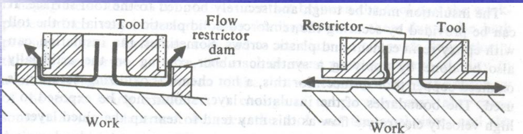
Fig. 6.46 Control of electrolyte flow by restrictor dams.
