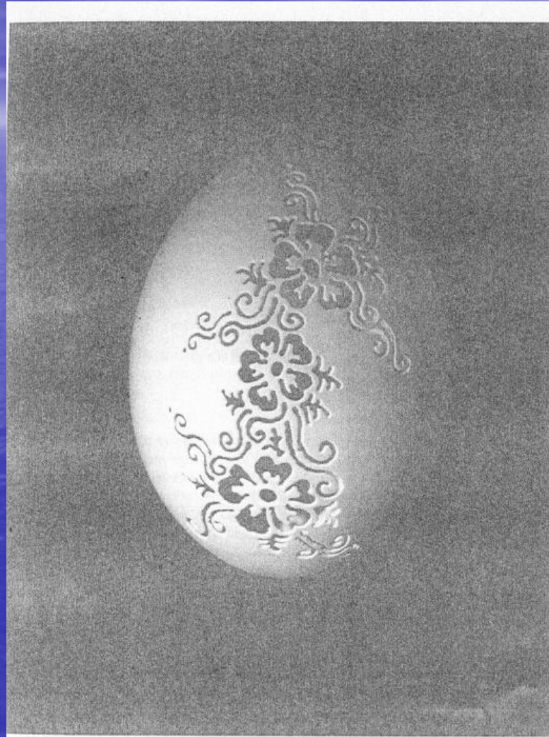
Figure 2.1 An AJM-machined egg shell showing the ability of the process to machine intricate shapes into brittle workpieces (Source: S. S. White Industrial Products, Pennwalt Corporation, Piscataway, NJ).
