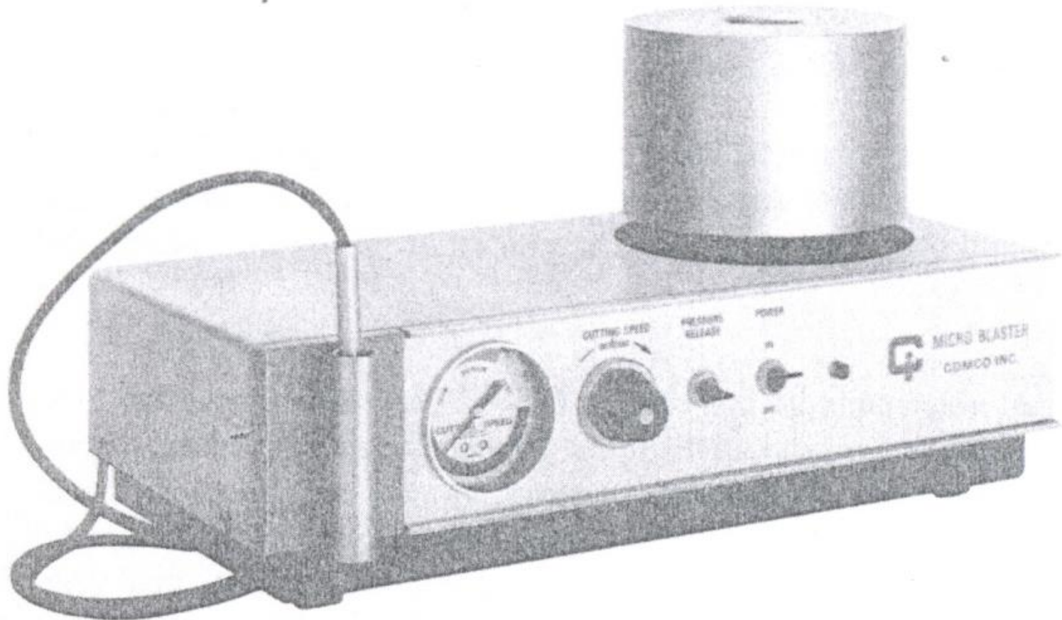
Figure 2.3 An AJM system showing main unit, powder hopper, and hand-piece (Source: Comco, Inc. Burbank, Calif).
