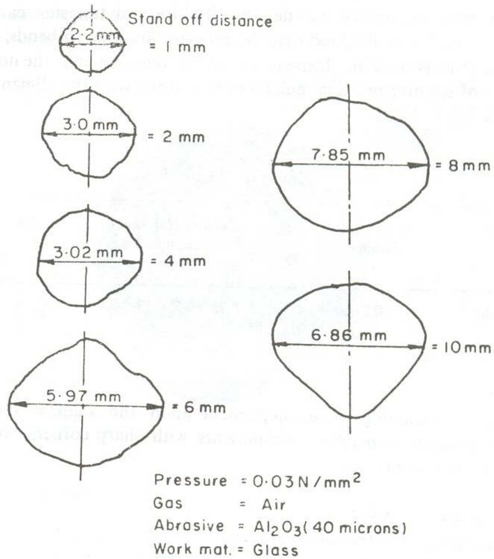
Fig. 2.22 Effect of stand off distance on the accuracy of shape produced
