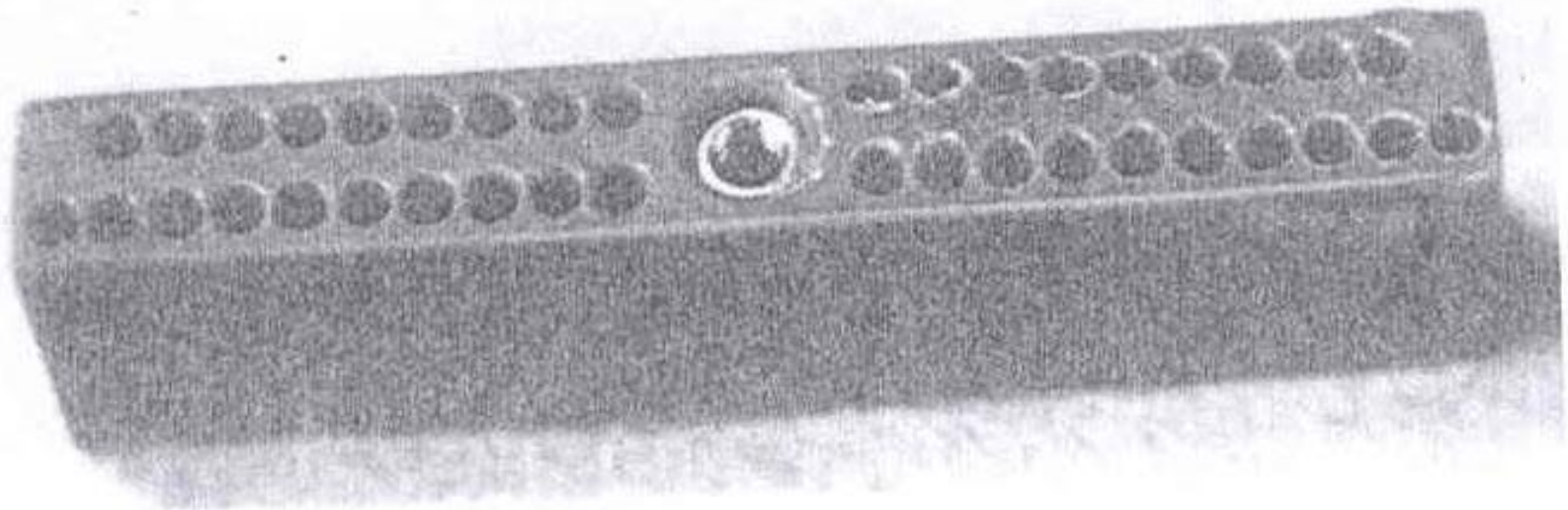
Figure 2.12 Plastic connector body showing condition before and after flash removal by AJM (Source: Comco, Inc., Burbank, Calif).
