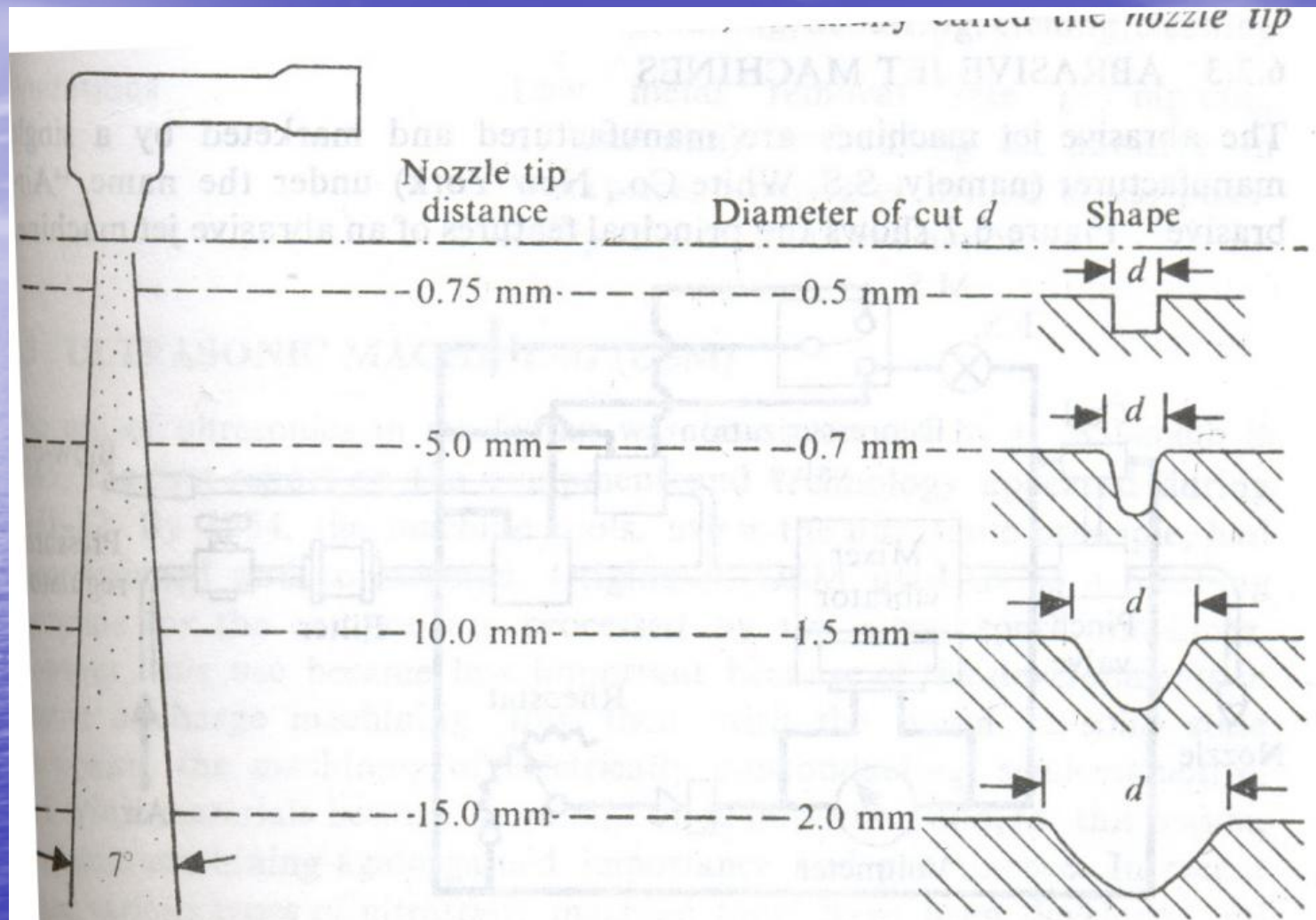
Fig. 6.5 Effect of nozzle tip distance on shape and size of cut.
